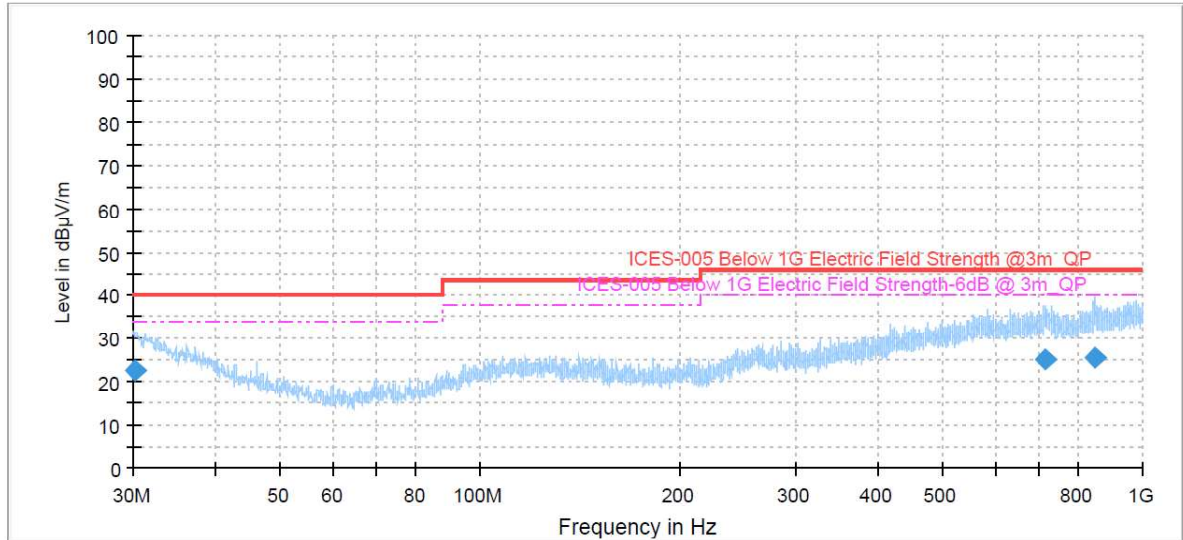
Figure 3: Spectral Diagrams, Radiated Emission, 30MHz-1000MHz, Horizontal polarization
