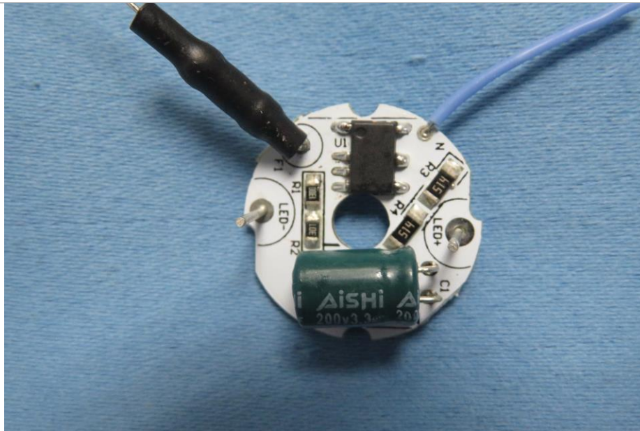
PCB view
