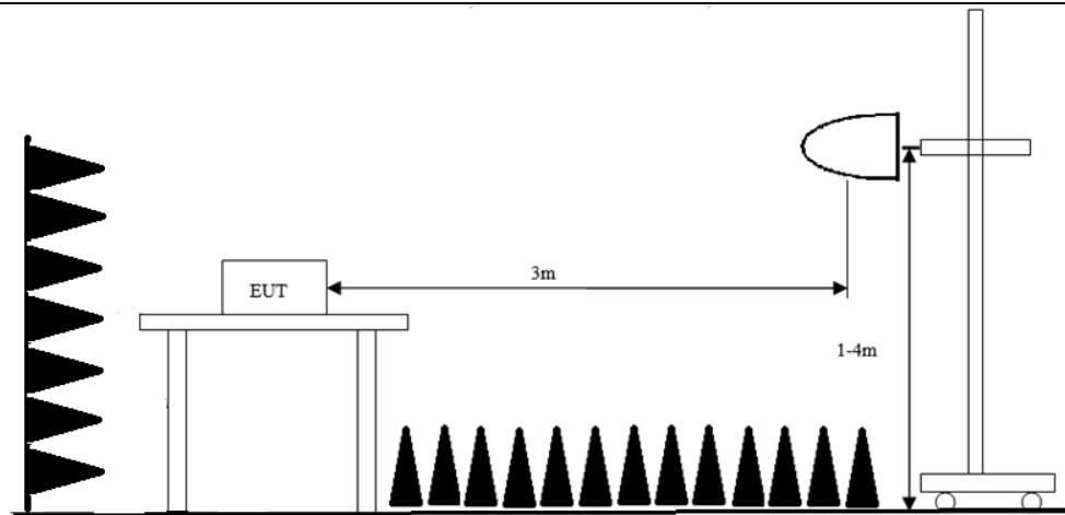
(Radiated emission 1-18 GHz)
