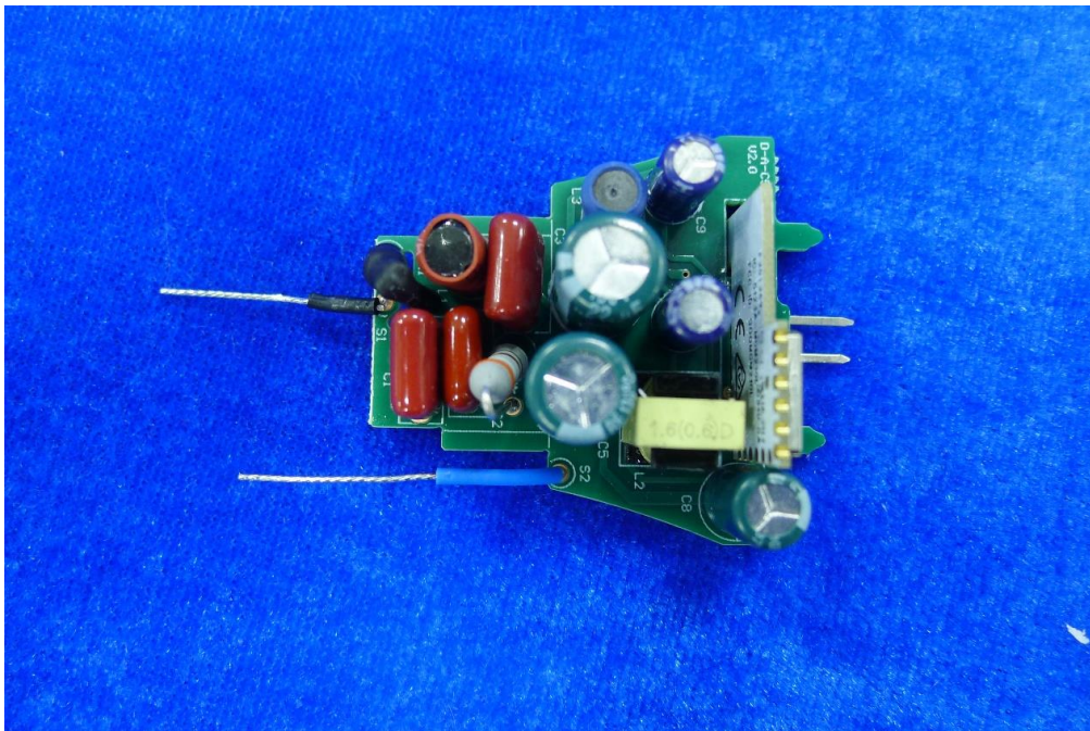
PCB
