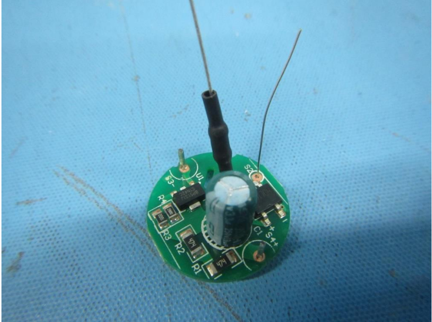
Photo 2 - Internal view
