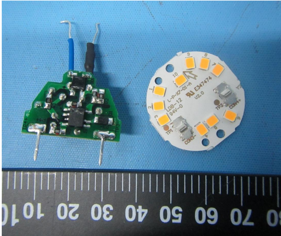
Photo 3 - Internal view
