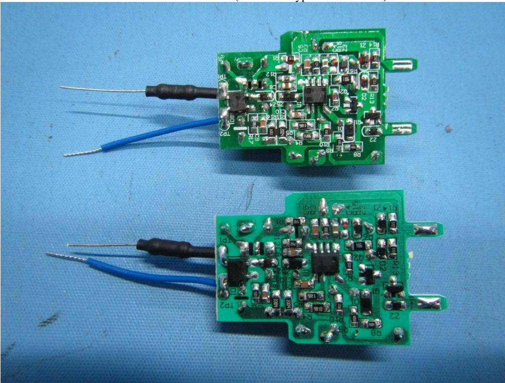
Photo 6 - Internal view (alternative type of driver PCB)
