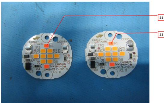
Photo 6 - Alternative LED PCB (Left - SAMSUNG; Right - SEOUL)
