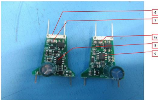
Photo 5 - Alternative driver PCB (Left - U1: BP5178FLD; Right - U1: SY59108N)
