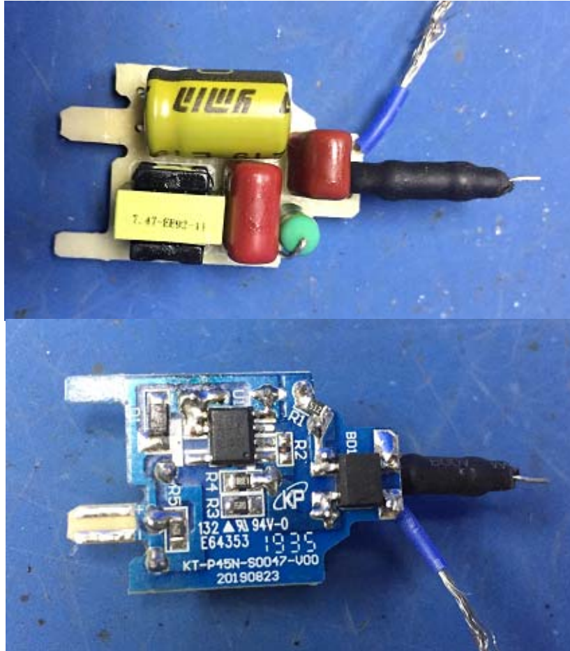
PCB view
