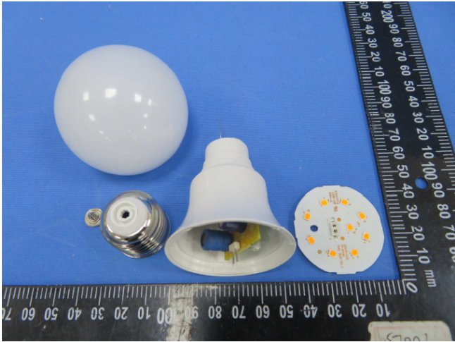
Exploded View
