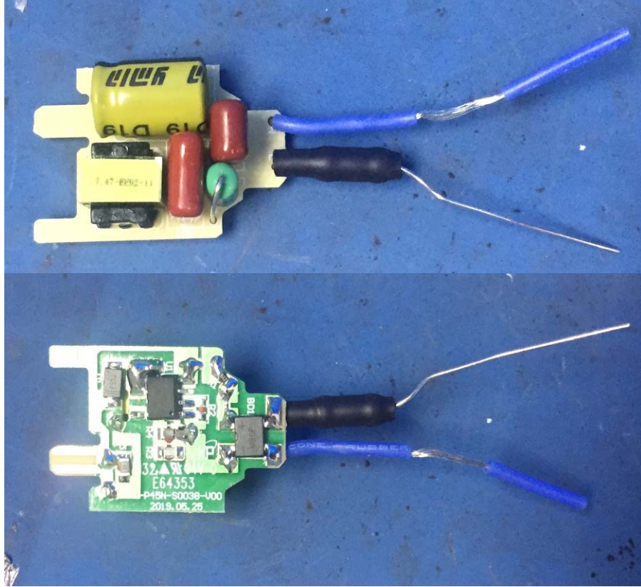
PCB view
