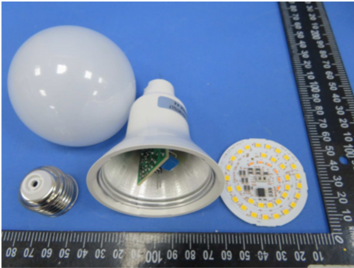
Exploded view
