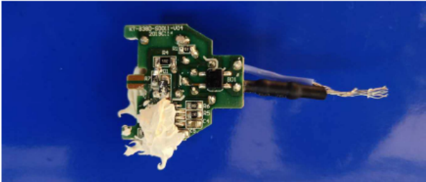
PCB top view
