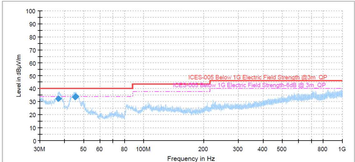
Figure 4: Spectral Diagrams, Radiated Emission, 30MHz-1000MHz, Vertical polarization Full Spectrum
