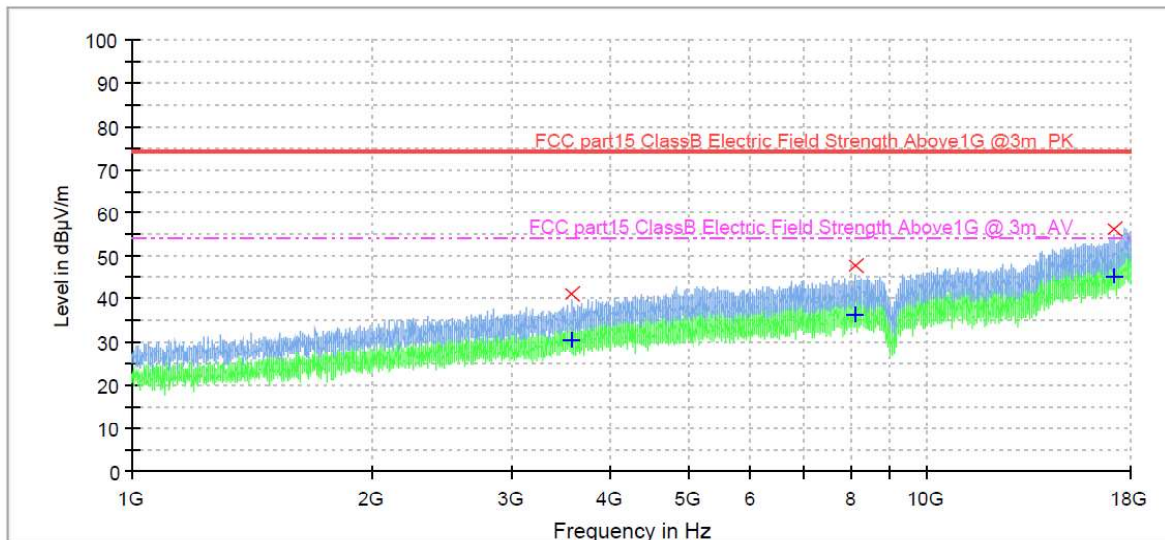
Figure 5: Spectral Diagrams, Radiated Emission, 1GHz-18GHz, Horizontal polarization
