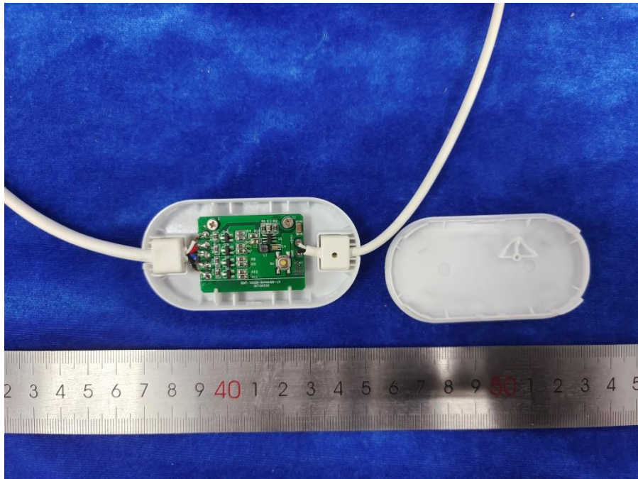
Inside control box
