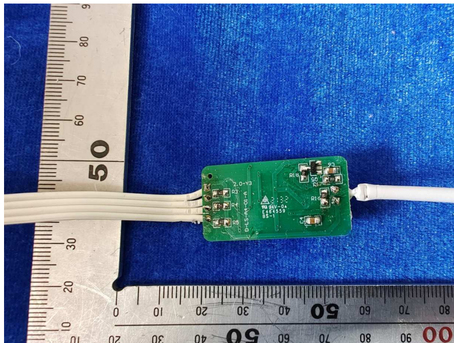
Controller PCB view
