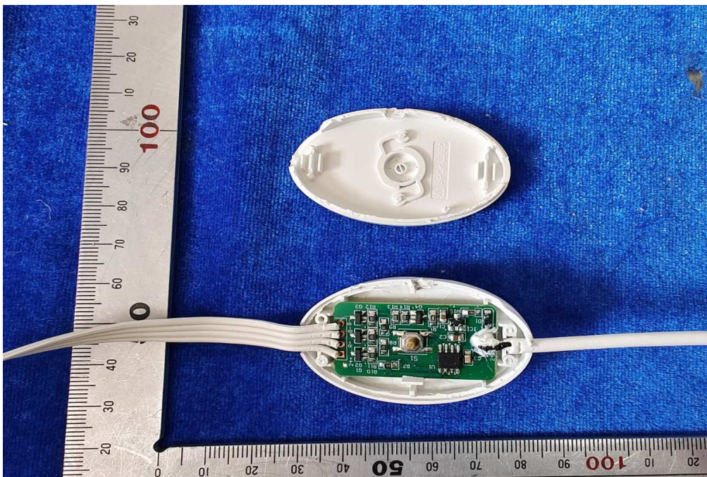
Inside Controller view
