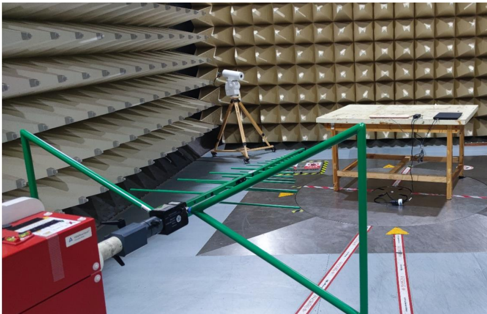
Photograph 2: Set-up for measurement of radiated emission
