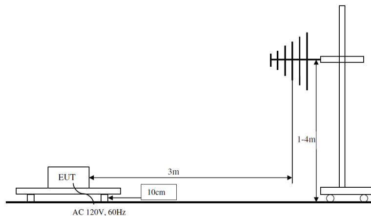
(Radiated emission)
