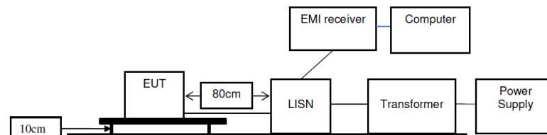
(Conducted emission)
