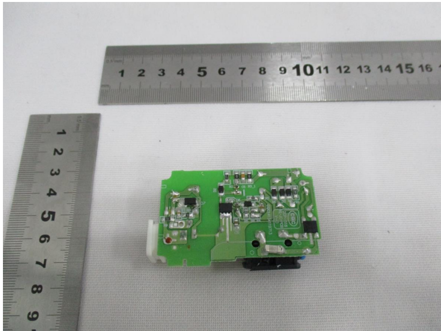
LED driver PCB
