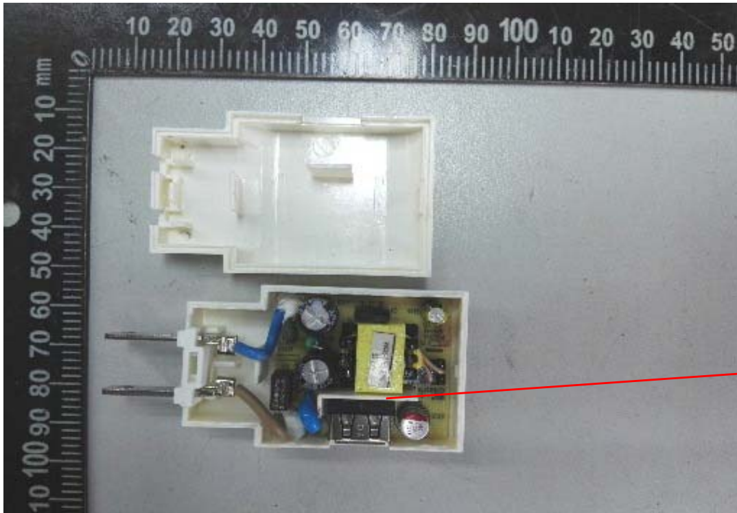
Photo 3 - Internal view
