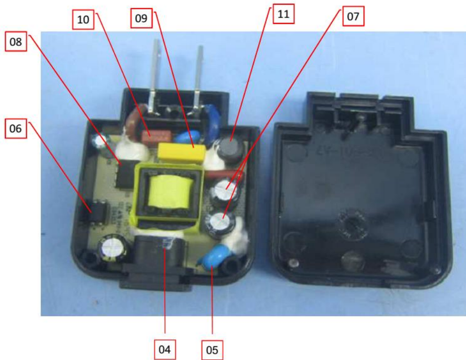
Photo no. 2 - Internal view of the Class 2 Power Supply, model KMV-***-***-NA-3
