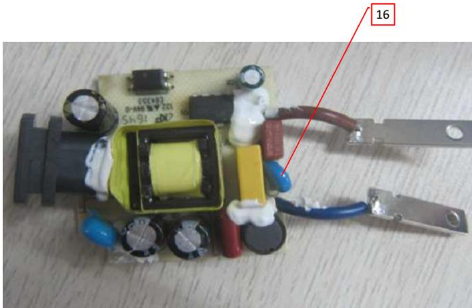
Photo no. 5 - Internal view of the Class 2 Power Supply, model KMV-***-***-NA-3
