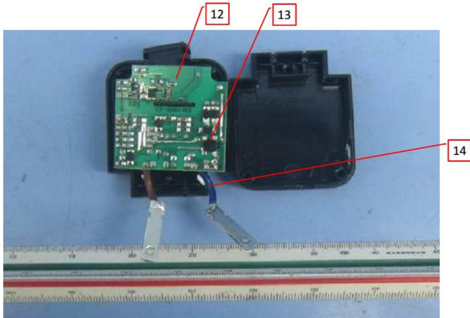
Photo no. 3 - Internal view of the Class 2 Power Supply, model KMV-***-***-NA-3
