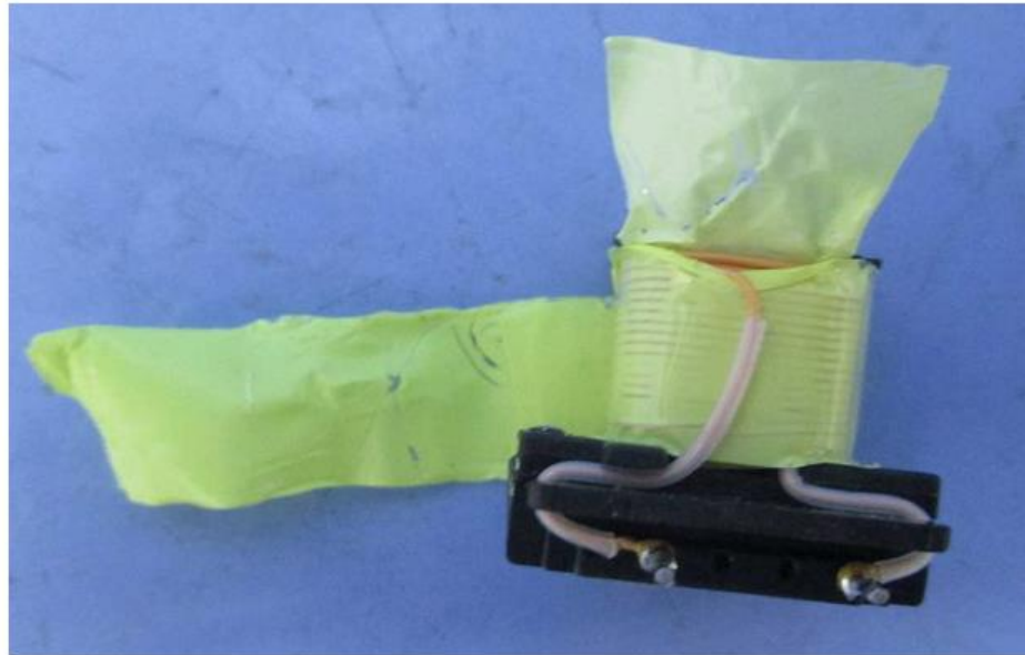
Photo no. 7 - Internal view of HF transformer for all models
