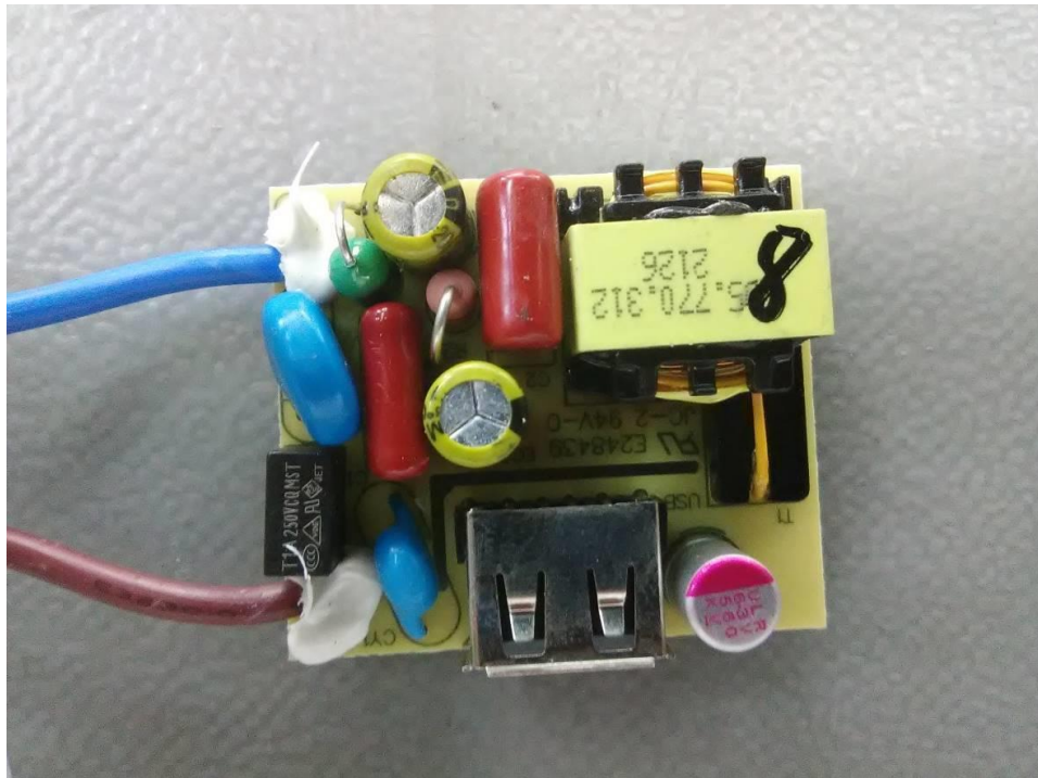
Photo 2 - PCB view
