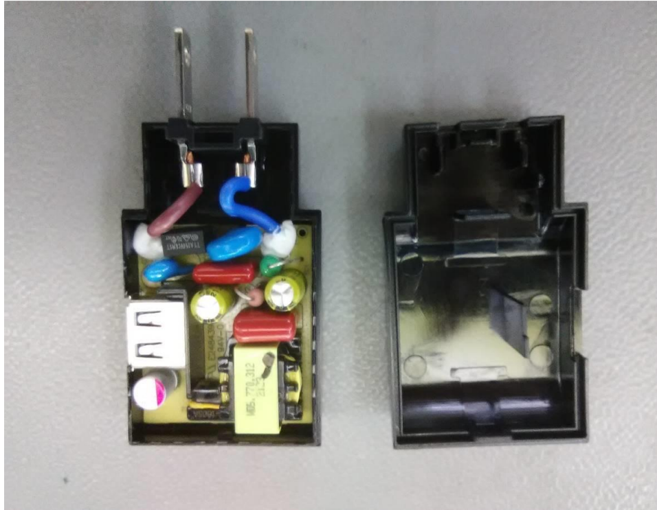
Photo 2 - PCB view
