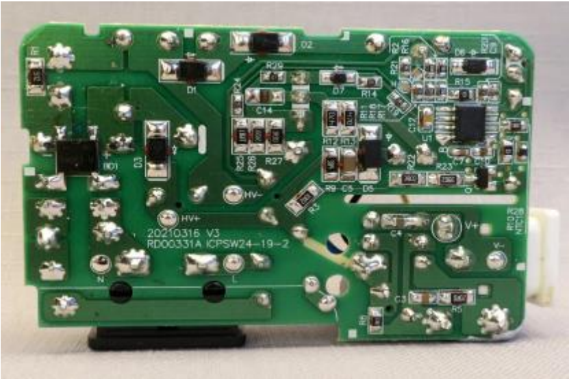
View of the PWB rear side
