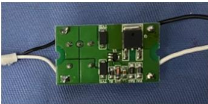
Control PCB(Back)
