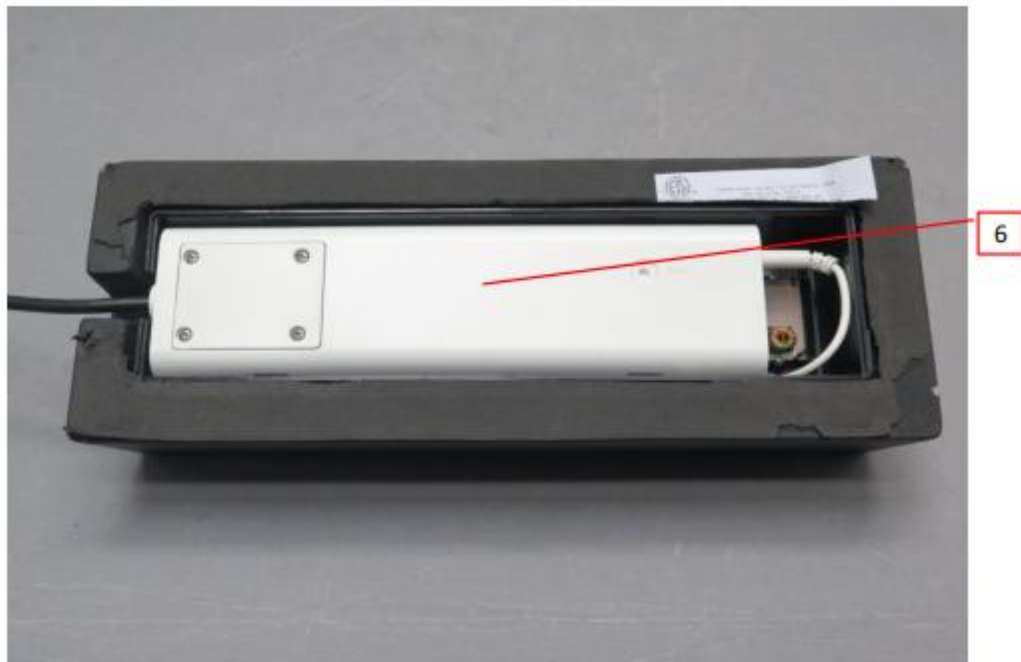
Photo 4 - Internal view
