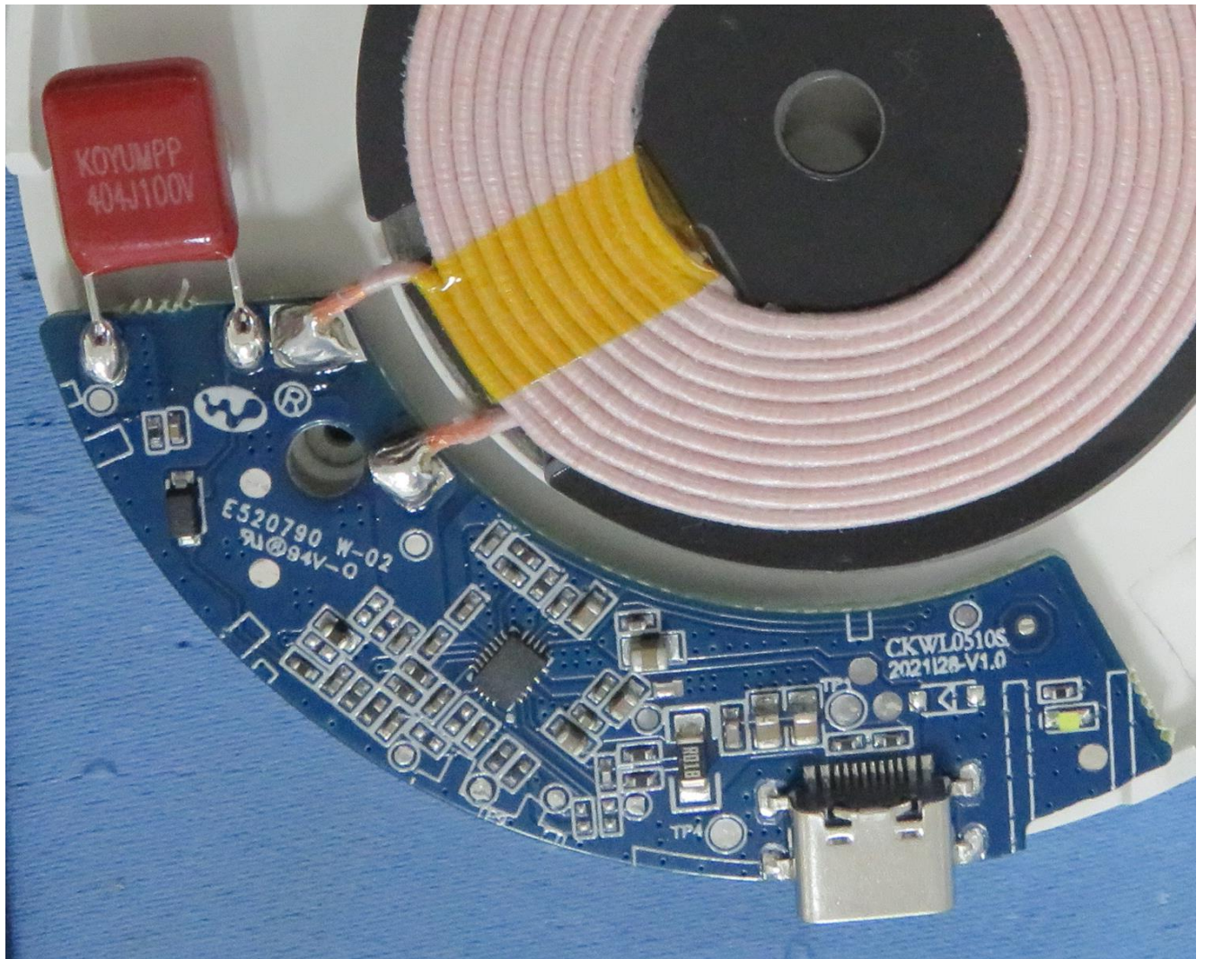
PCB View
