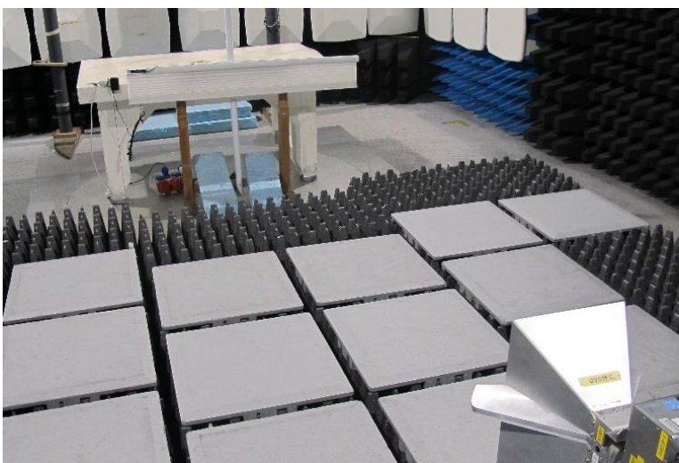
Test set up radiated emission 1 GHz – 13 GHz
