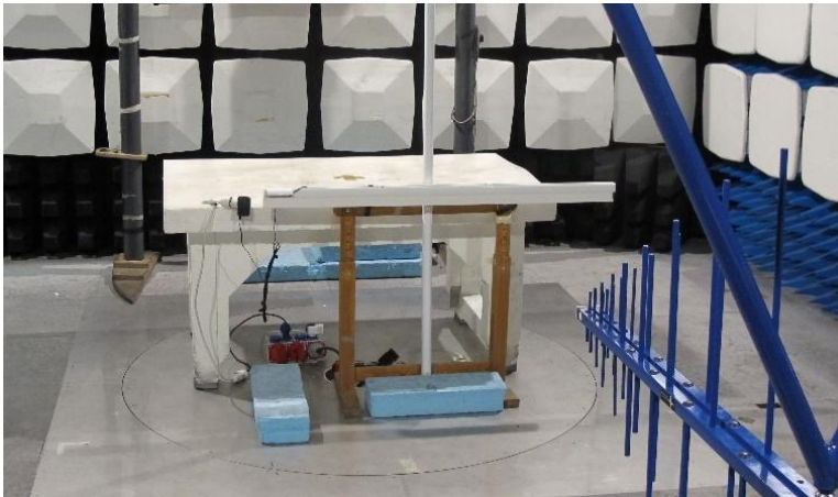
Test set up radiated emission 30 MHz – 1 GHz
