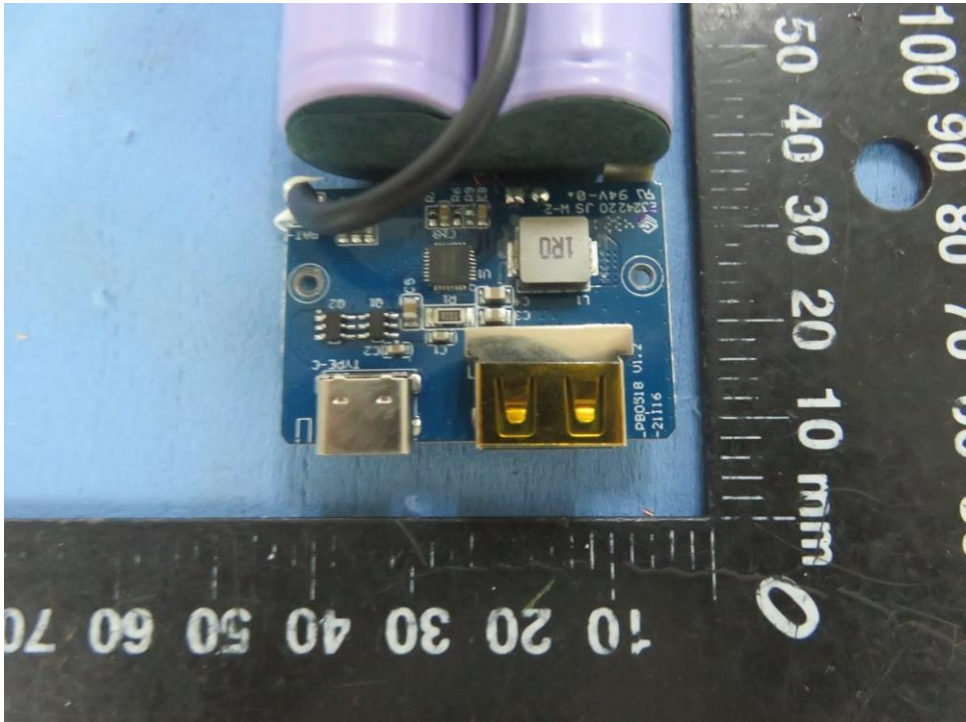
PCB view
