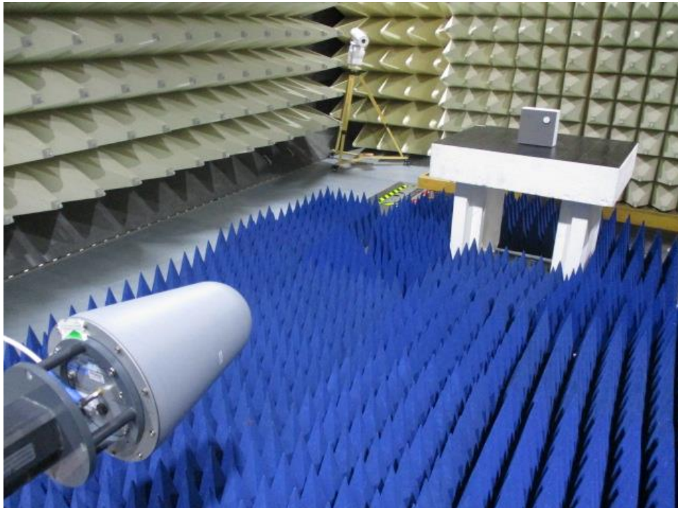
Photograph 3: Set-up photo for Radiated Emission, 1GHz - 6GHz
