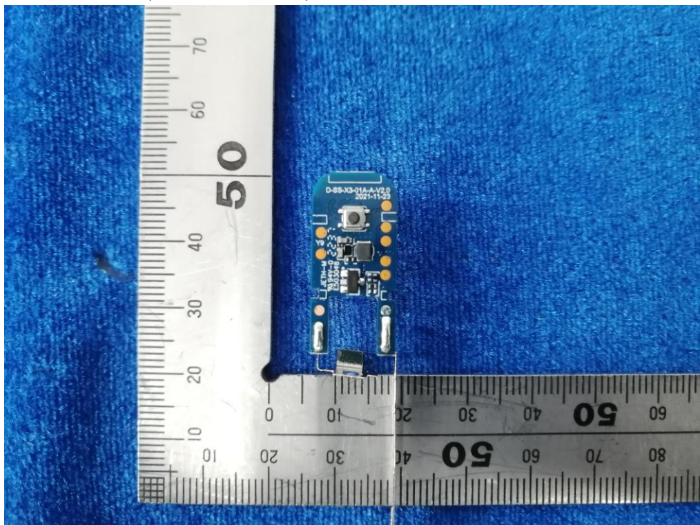
Bild / Picture 4: PCB view with U3 (IC model MAX17224)
