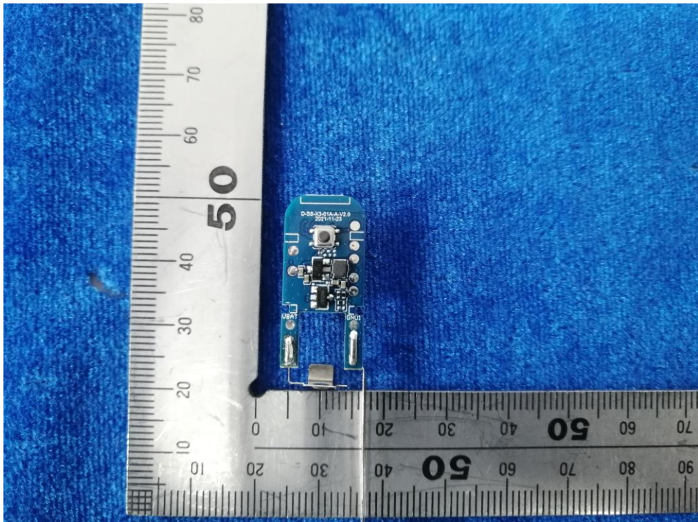
Bild / Picture 6: PCB view with U3 (IC model OC6811)
