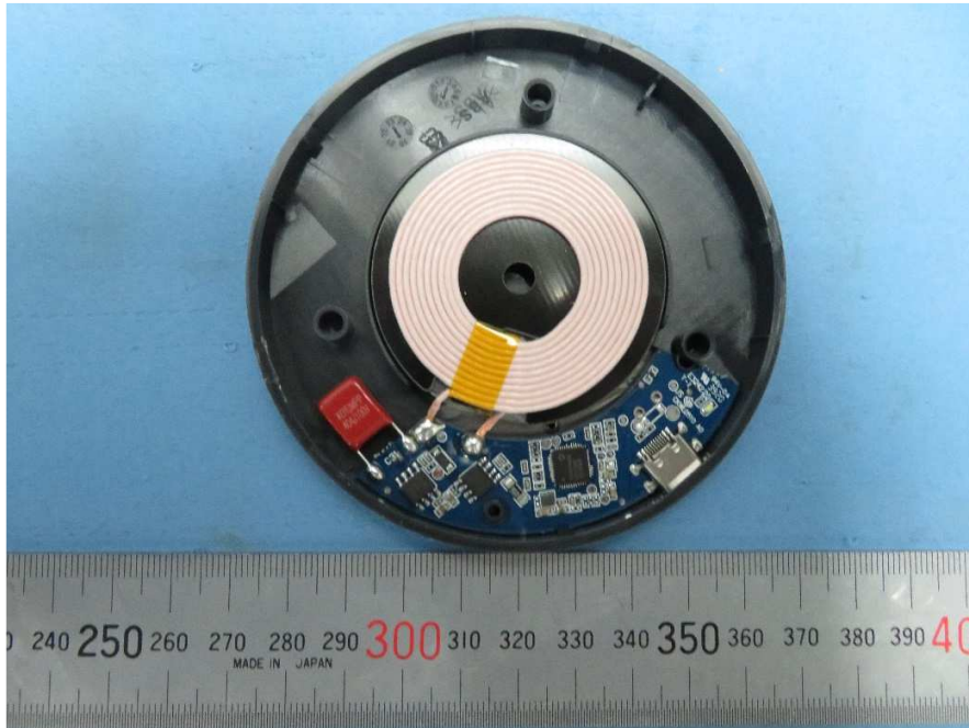
Internal view
