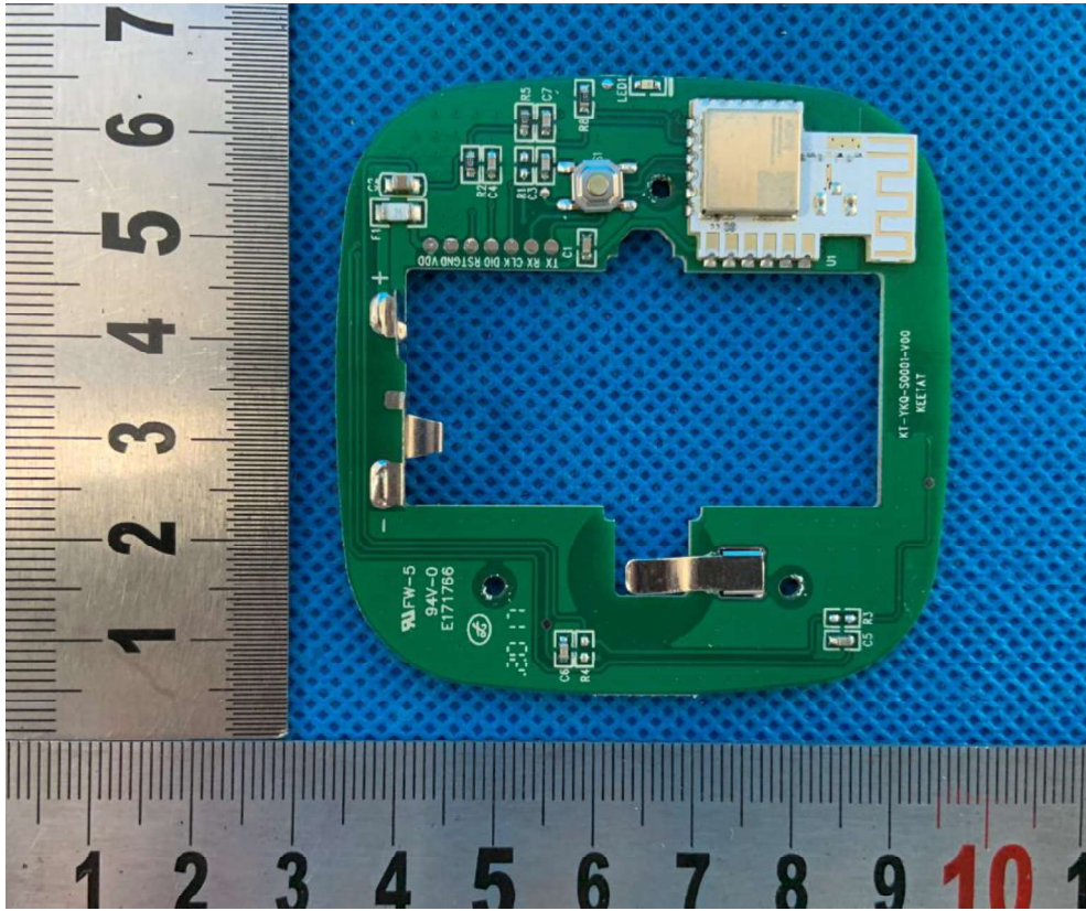
Picture 11 – Internal view
