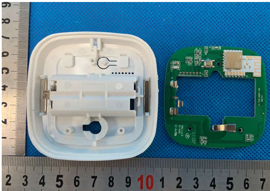
Picture 10 – Internal view
