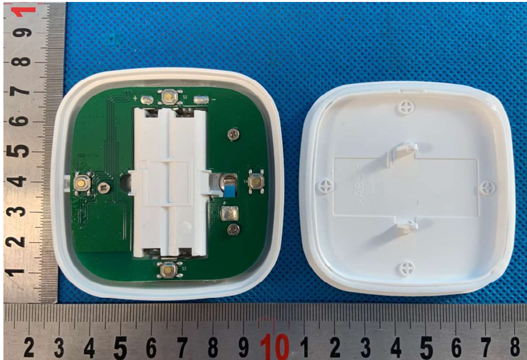
Picture 7 – Internal view
