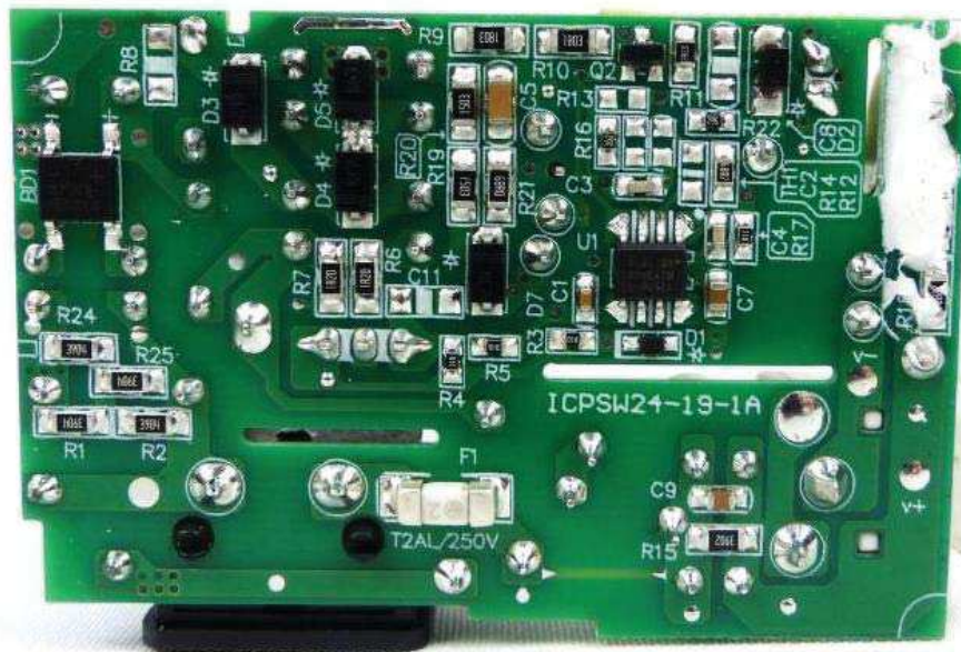
Rear view of adapter PCB (ICPSW24-19-1A)
