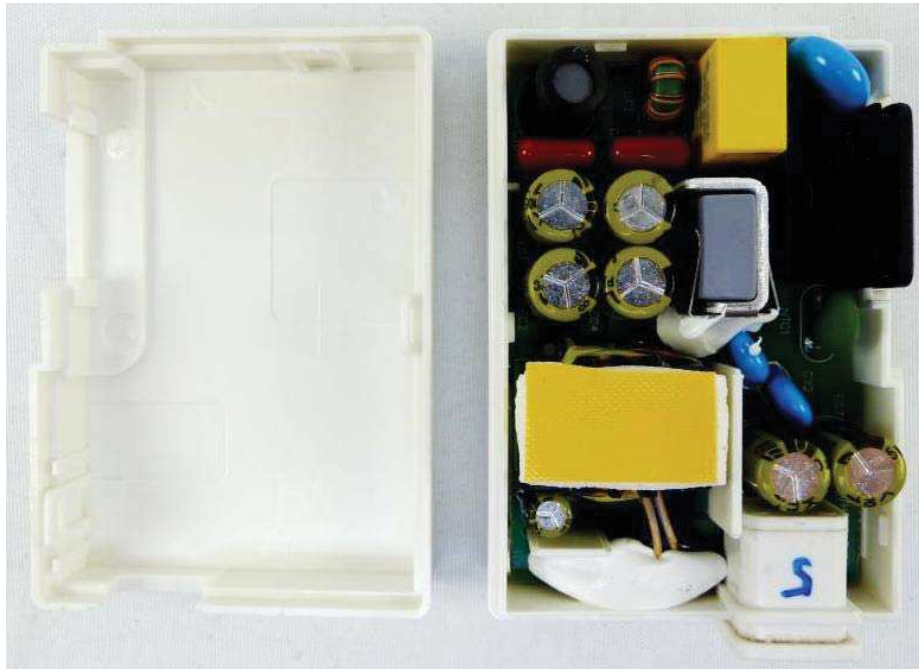
Inner view of adapter (ICPSW24-19-1A)
