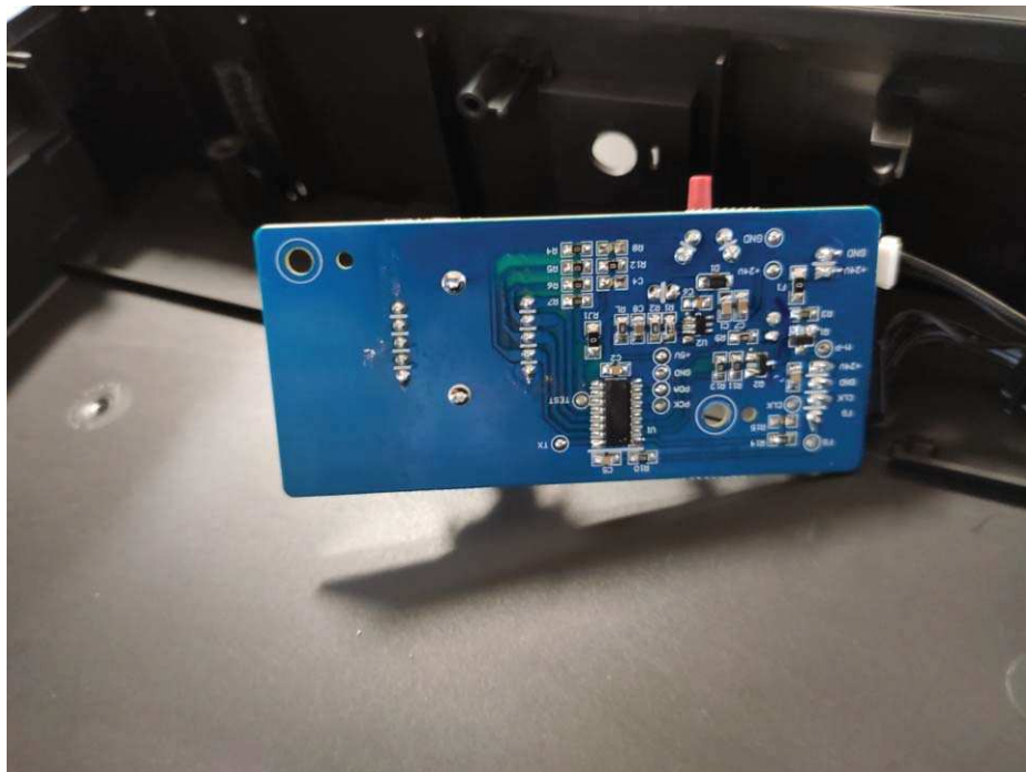
Control board view
