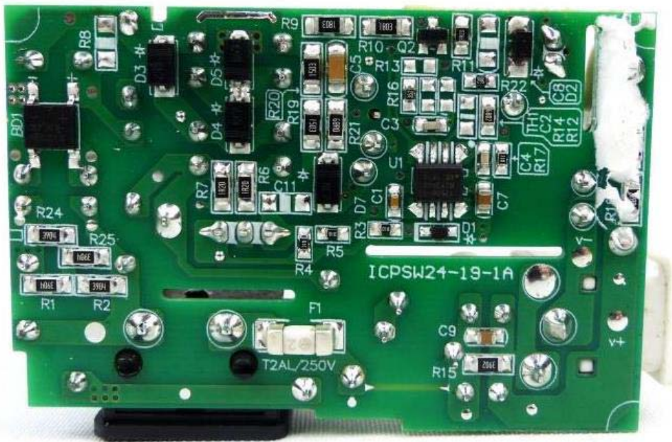
Rear view of adapter PCB (ICPSW24-19-1A)
