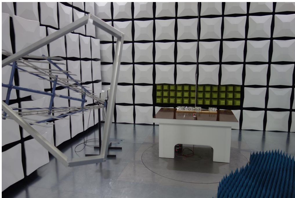
Photo of test setup 30MHz – 1GHz
