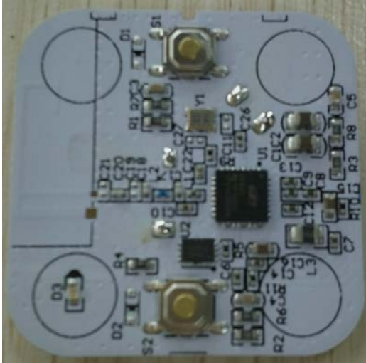
E1743 and E1766 PCB (Primary and secondary side)
