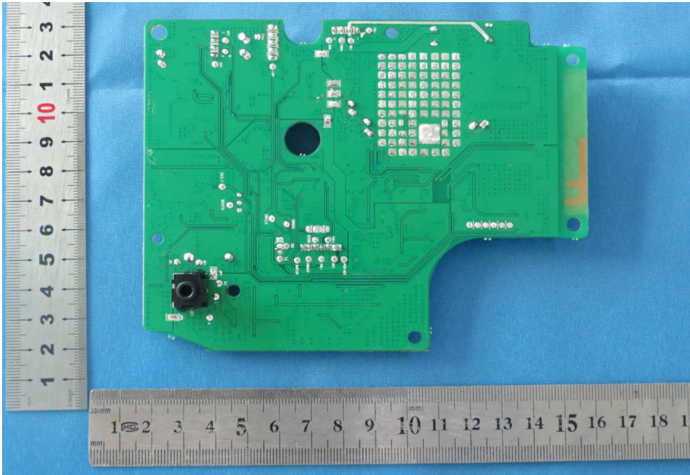
Picture 5- Mainboard
