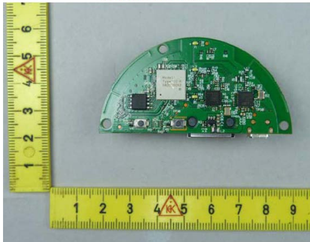
Internal view of E1526 TRÅDFRI
