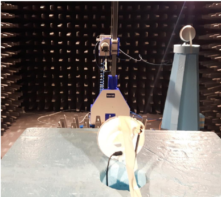
Test set up radiated emission > 18 GHz
