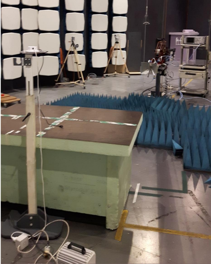
Test set up radiated emission 1 GHz – 18 GHz
