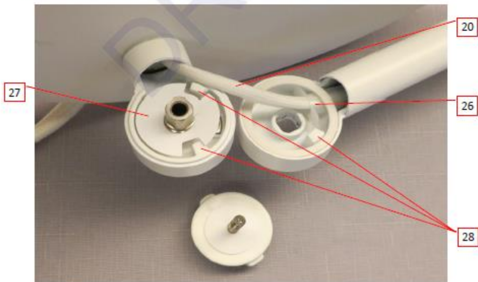
Photo 14 - Internal view of the lower joint
