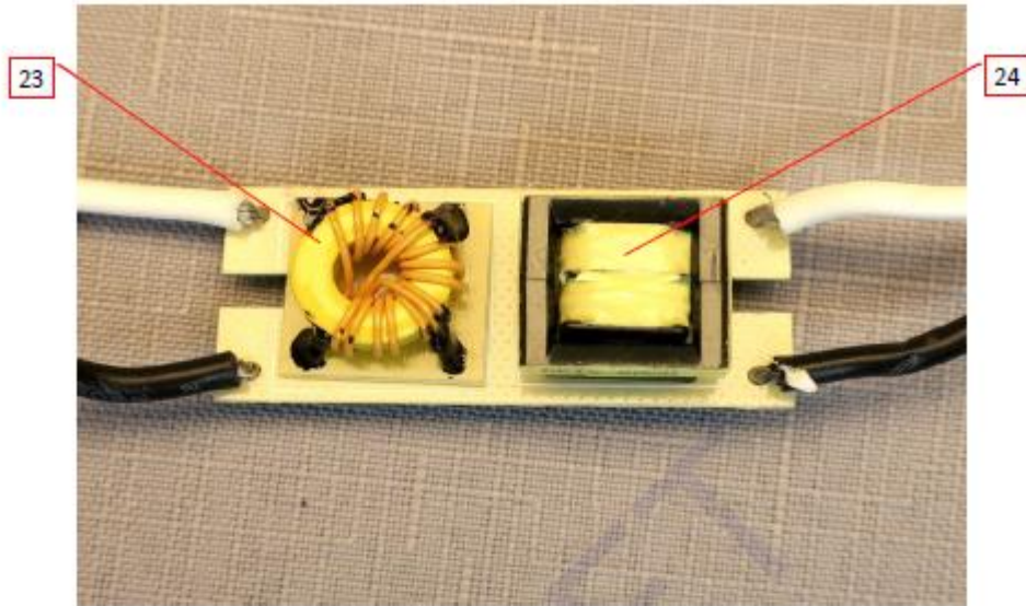
Photo 11 - View of line filter (removed)
