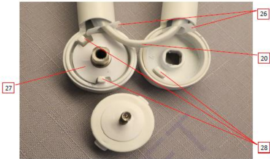
Photo 13 - Internal view of the upper joint
