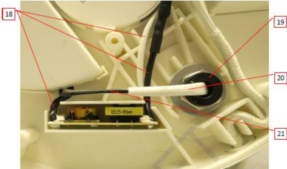
Photo 9 - Internal view (line filter cover removed)
