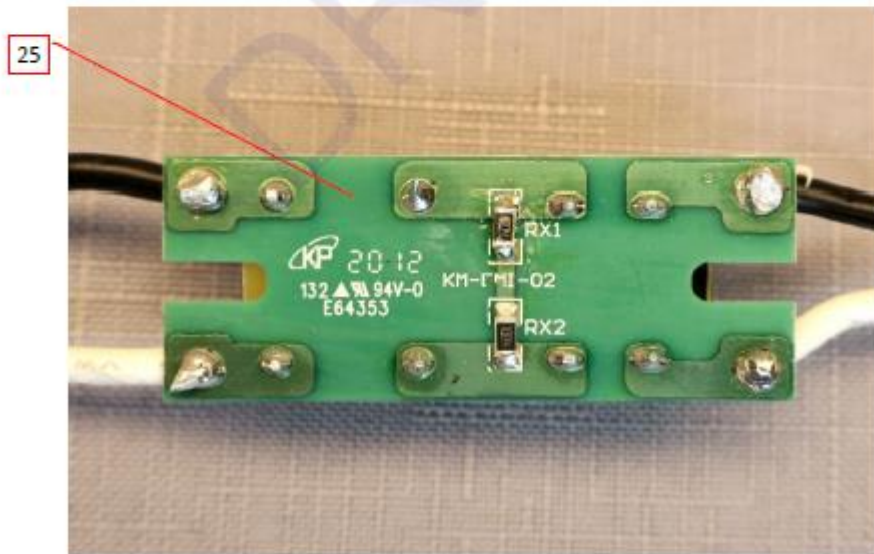
Photo 12 - View of line filter (removed)
