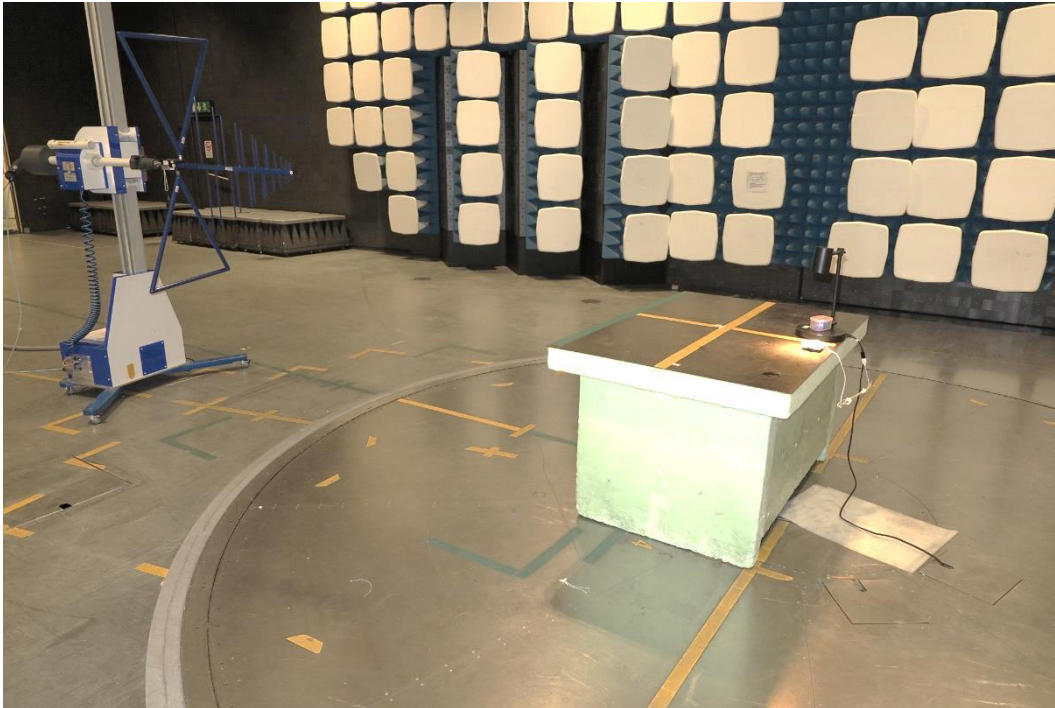
Test set up radiated emission 30 MHz – 1 GHz
