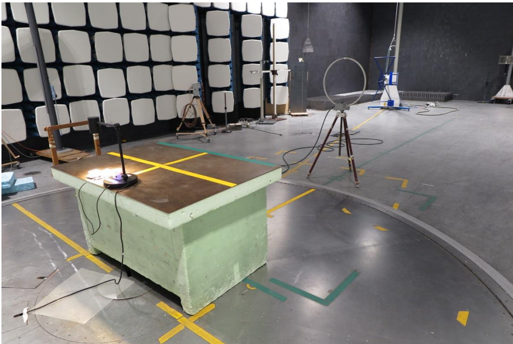
Test set up radiated emission 0.009 MHz – 30 MHz
