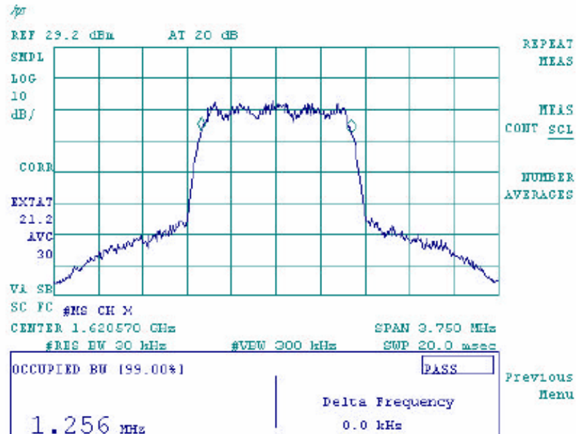
Channel 9 Occupied Bandwidth
