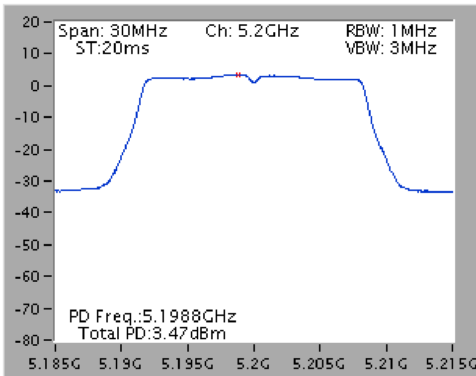
Power Density Plot on Configuration IEEE 802.11a / Ant. 0 + Ant. 1 / 5200 MHz
