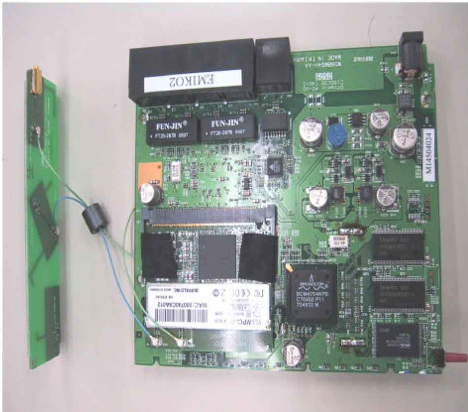
Front View of Print Circuit Boards Put Off Enclosure
