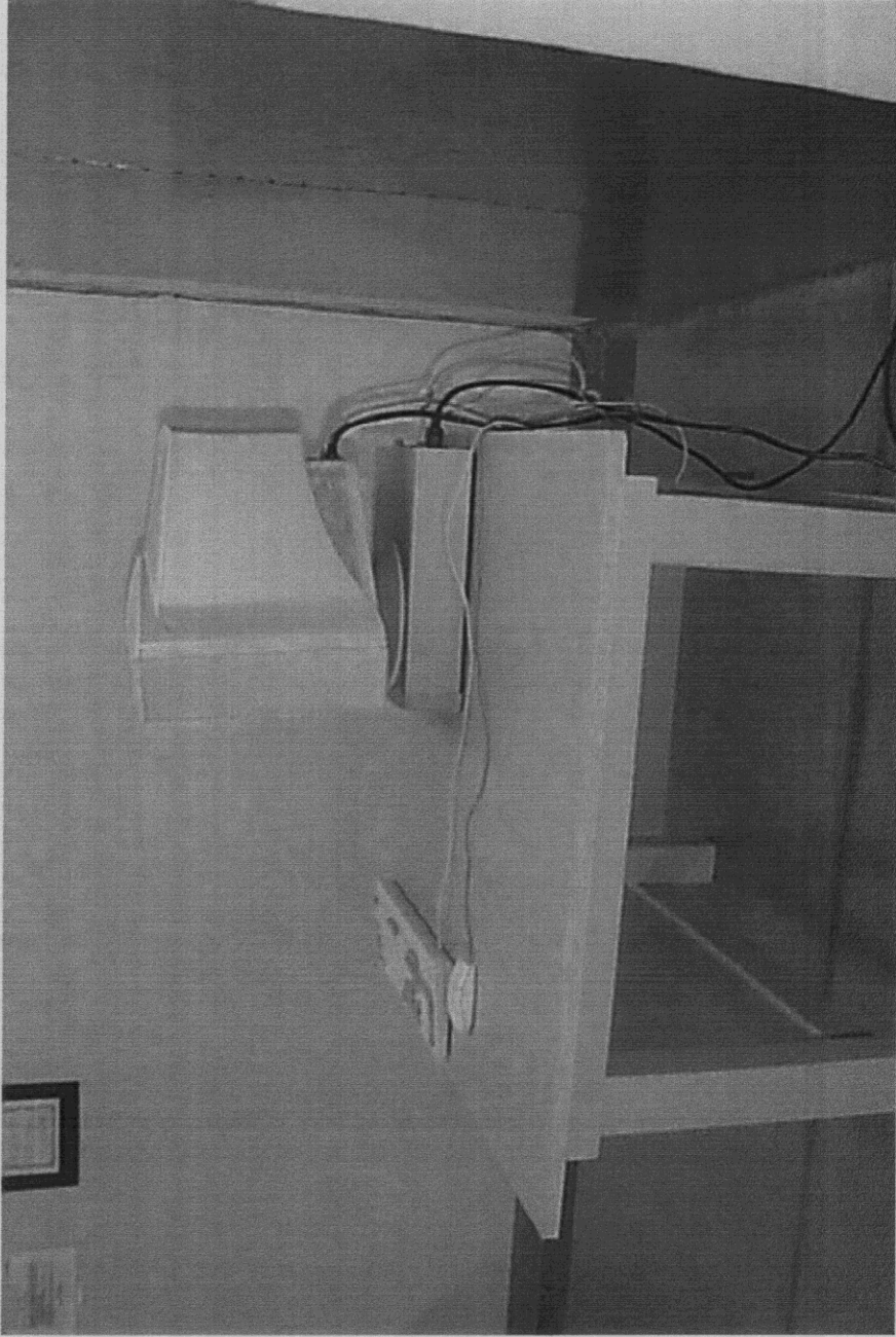
Conducted Emission Test Set-up - Rear View
