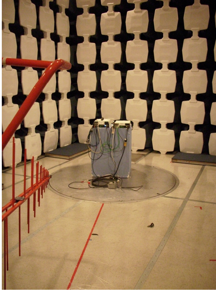
Radiated emission measurements below 1GHz - Front
