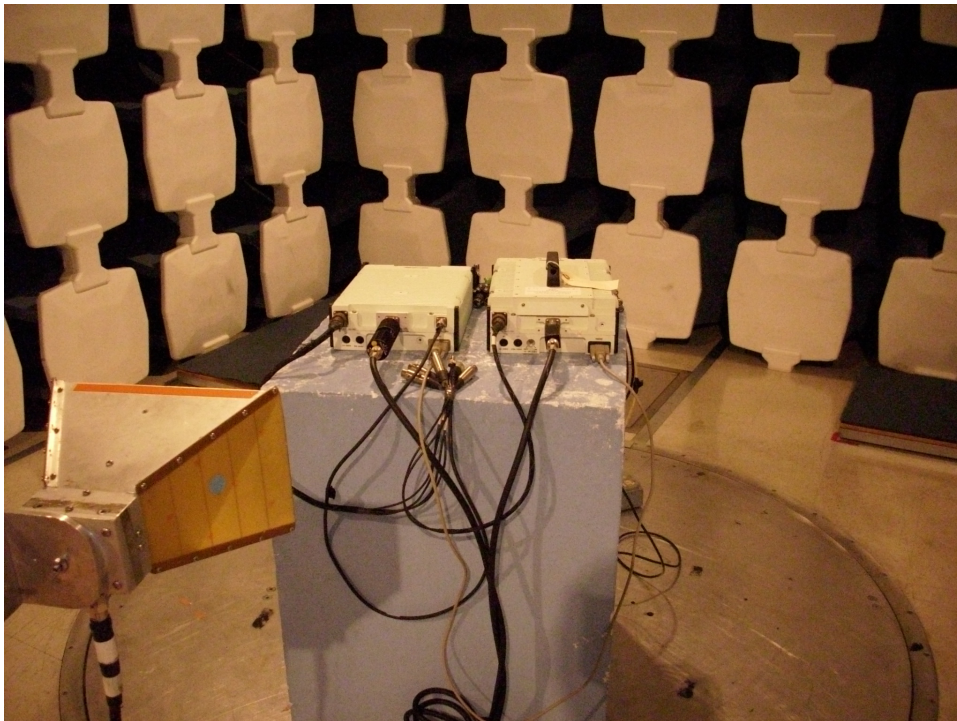
Radiated emission measurements above 1GHz - Rear
