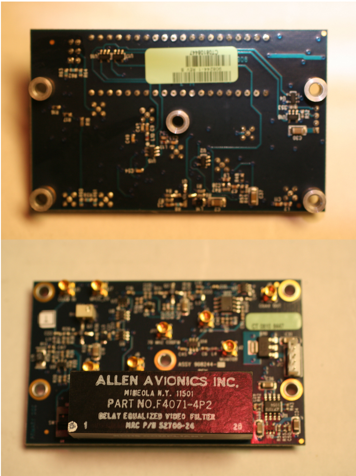
IF Board
