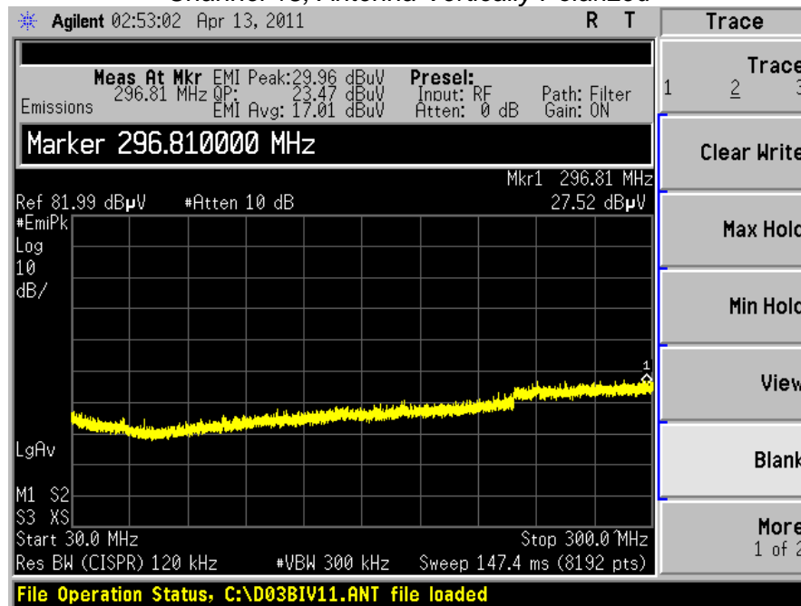
Channel 18, Antenna Vertically Polarized
