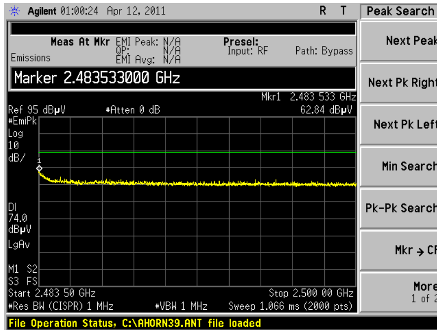
Dipole Antenna Channel 26 Power Level 9
