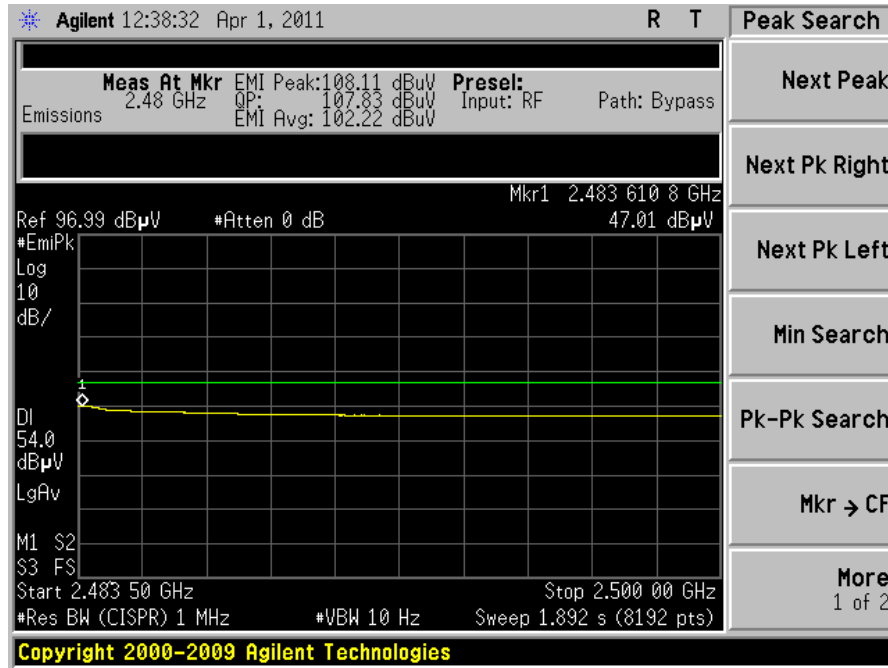
Chip Antenna Channel 25 Power Level 20
