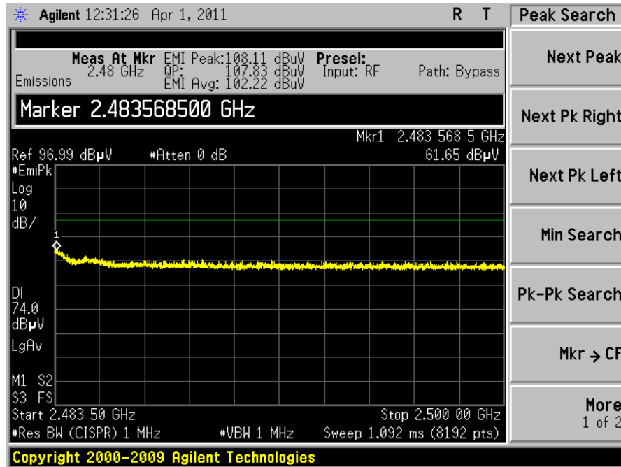
Chip Antenna Channel 26 Power Level 13
