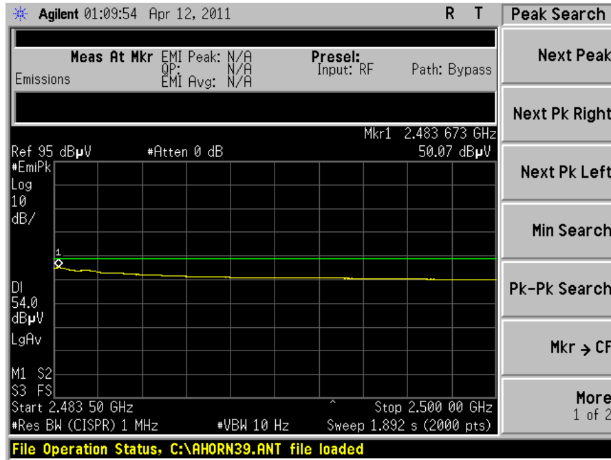
Dipole Antenna Channel 25 Power Level 20
