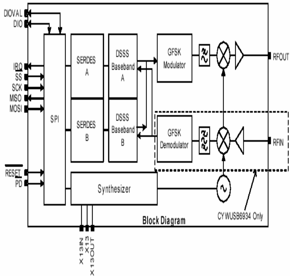
Figure 1. WirelessUSB LS Block Diagram
