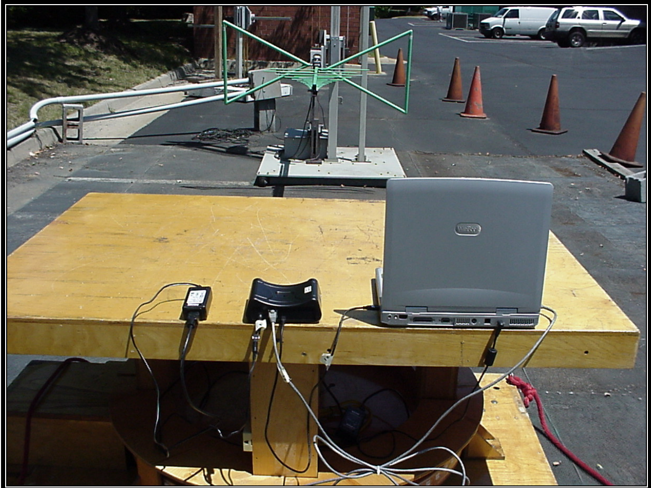
Photograph 14: Radiated Testing – Back View AC Adapter
